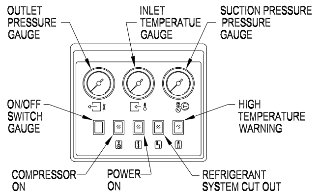
INSTRUMENT PANEL
