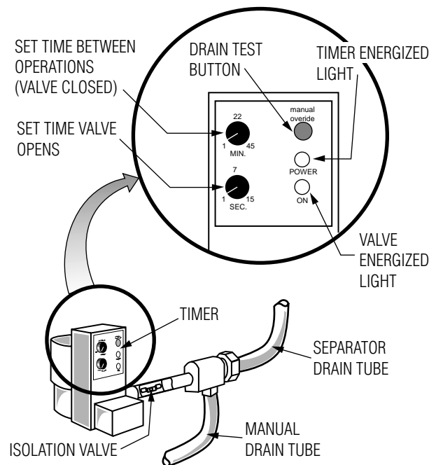
ELECTRIC ASSEMBLY
