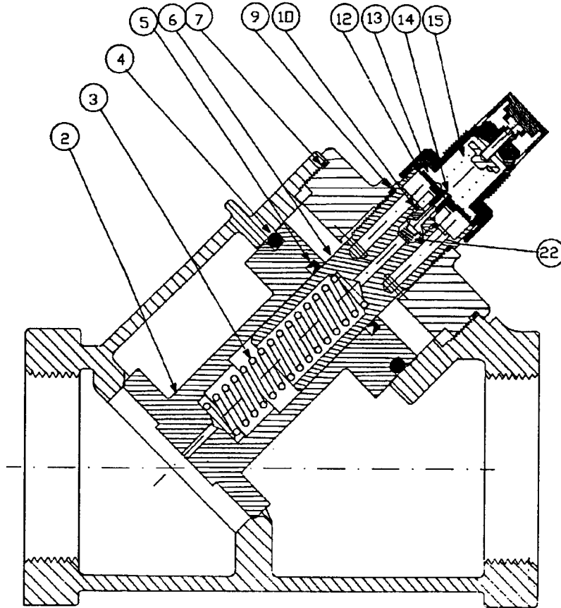
MINIMUM PRESSURE VALVE - 201ECM257
